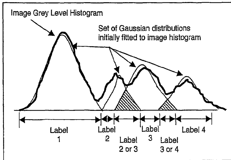
Figure 4; Hidden Markov Random Field Segmentation
