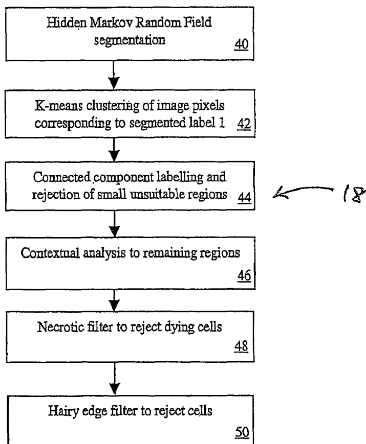
Figure 2 Mitosis feature cueing
