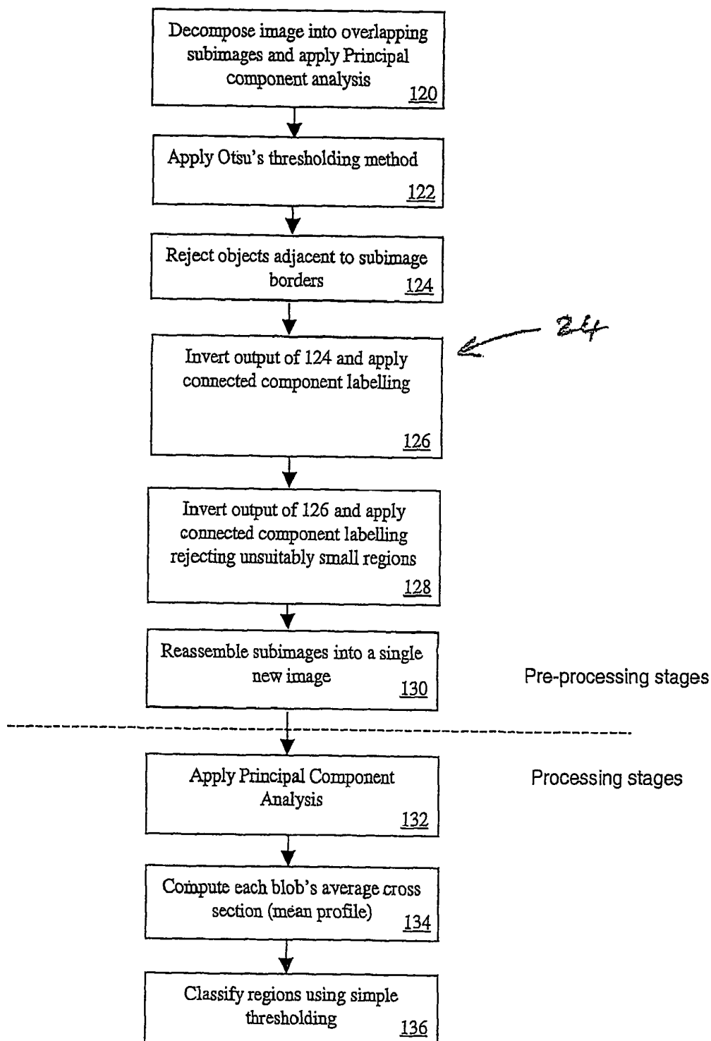
Figure 6 Mitosis feature detection process
